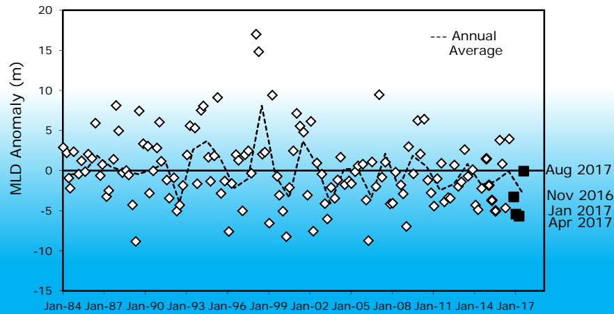
Mixed Layer Depth Anomaly (CalCOFI Std Grid) 198401-201708
