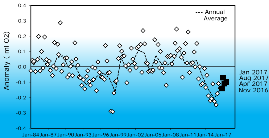
Mixed Layer Oxygen Anomaly (CalCOFI Std Grid) 198401-201708
