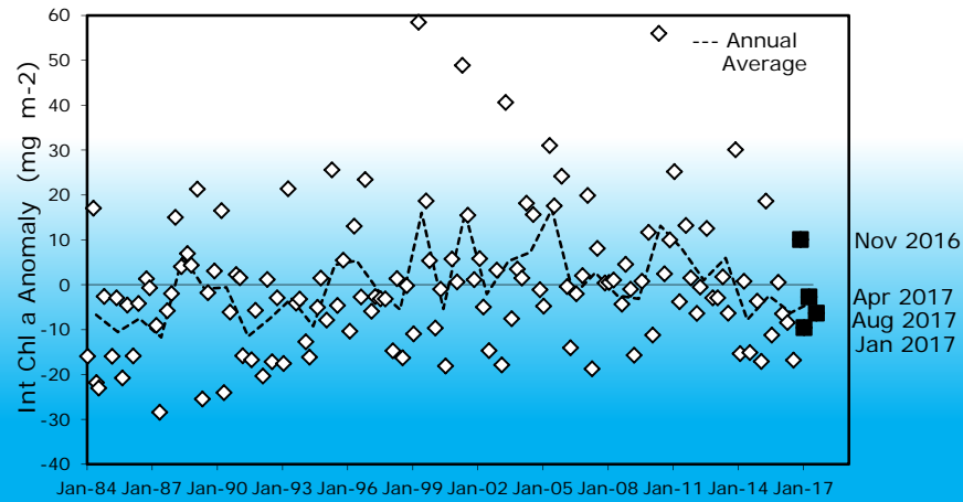
M.L. Integrated Chl-a Anomaly(CalCOFI Std Grid) 198401-201708
