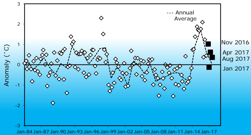
Mixed Layer Temp Anomaly (CalCOFI Std Grid) 198401-201708
