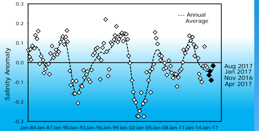
Mixed Layer Salinity Anomaly (CalCOFI Std Grid) 198401-201708
