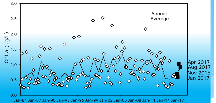
Mixed Layer Chl-a Avg (CalCOFI Std Grid) 198401-201708
