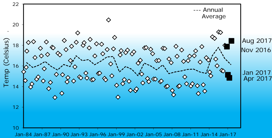
Mixed Layer Temp Avg (CalCOFI Std Grid) 198401-201708
