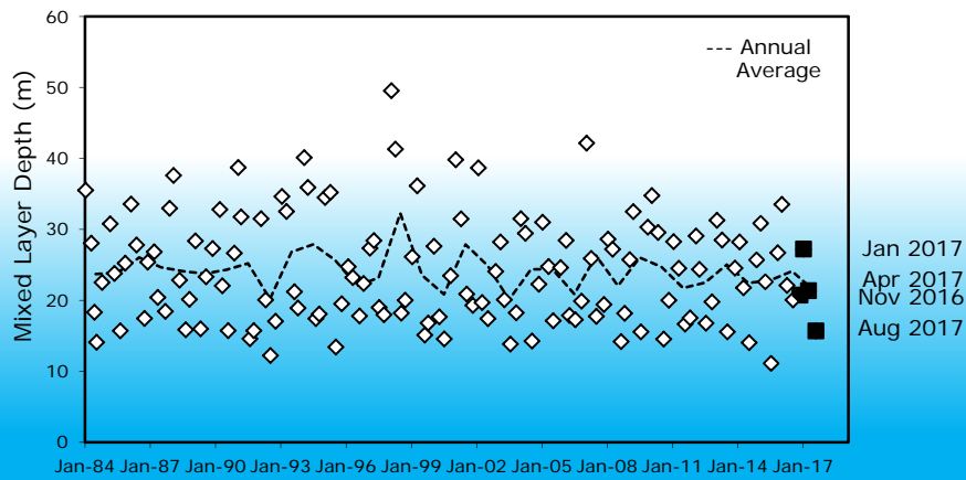
Avg Mixed Layer Depth (CalCOFI Std Grid) 198401-201708
