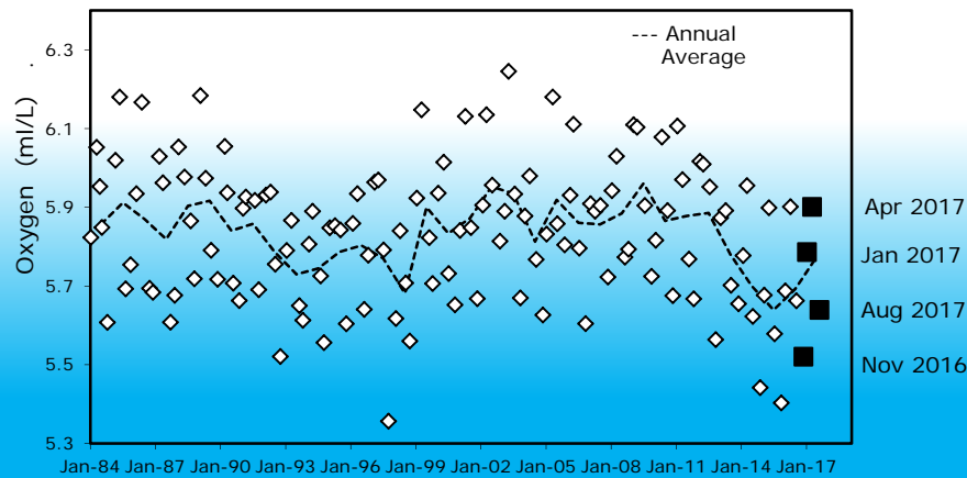
Mixed Layer Oxygen Avg (CalCOFI Std Grid) 198401-201708
