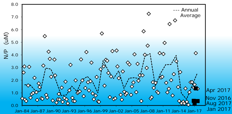
Mixed Layer N-P Ratio Avg (CalCOFI Std Grid) 198401-201708
