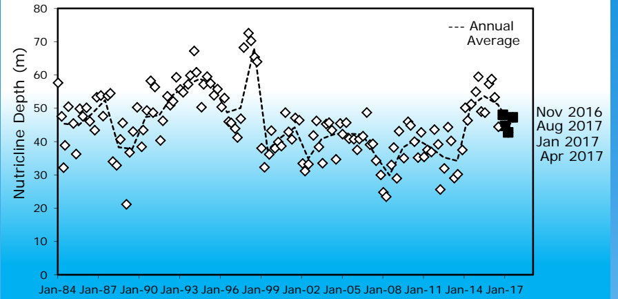
ML Nutricline Depth Avg (CalCOFI Std Grid) 198401-201708
