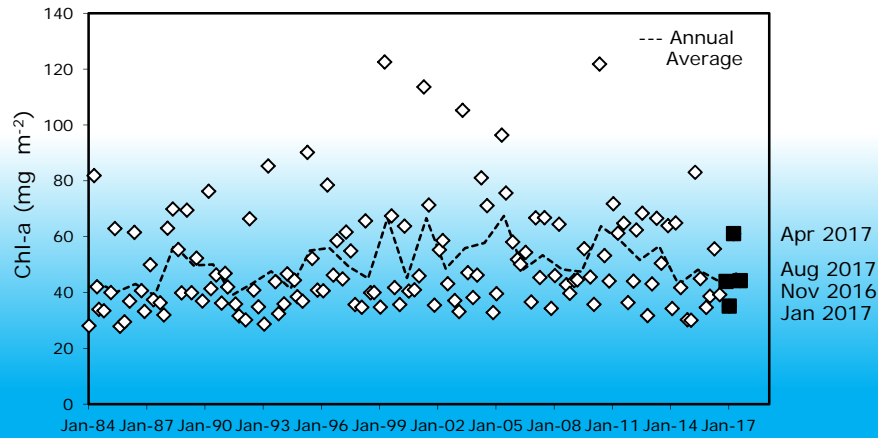
ML Chl-a Standing Stock Avg (CalCOFI Std Grid) 198401-201708
