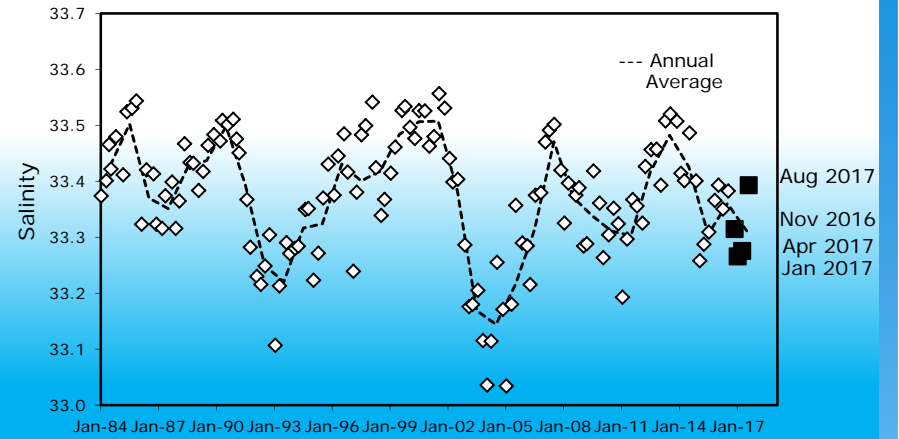
Mixed Layer Salinity Avg (CalCOFI Std Grid) 198401-201708
